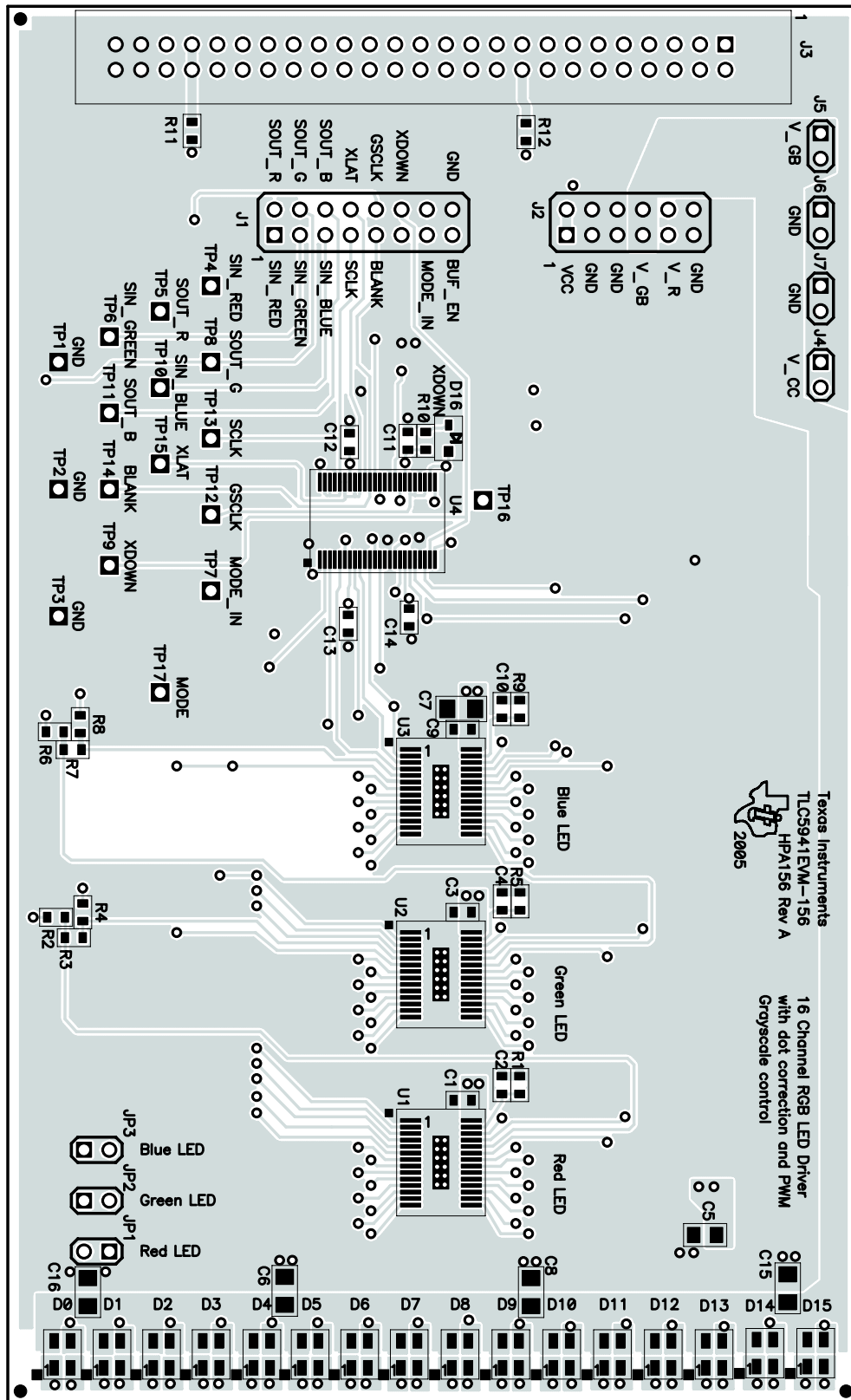
Figure 2. Assembly Layer
