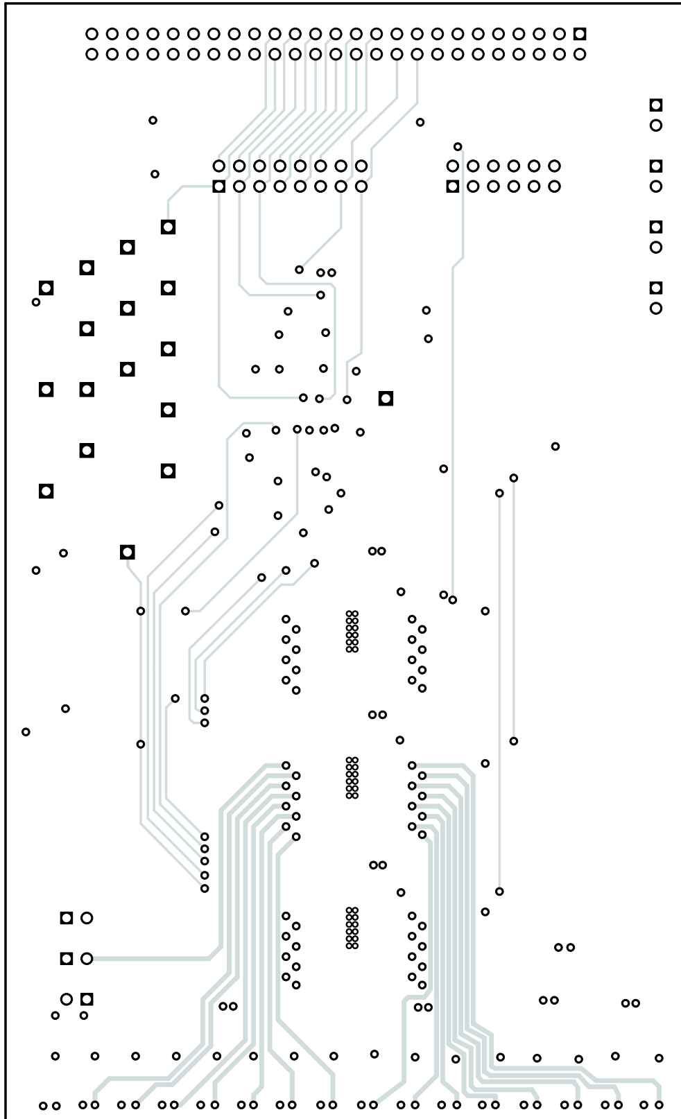
Figure 5. Layer 3 Routing
